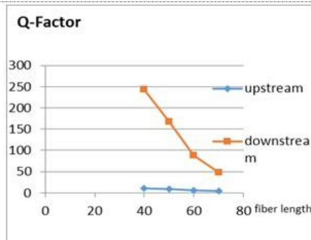
Figure 5 Comparison of Q factor for 5Gbps and 10Gbps BPON system
