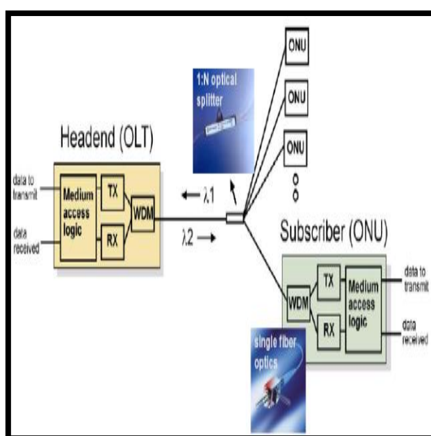
Figure 1 Basic PON Configurations
