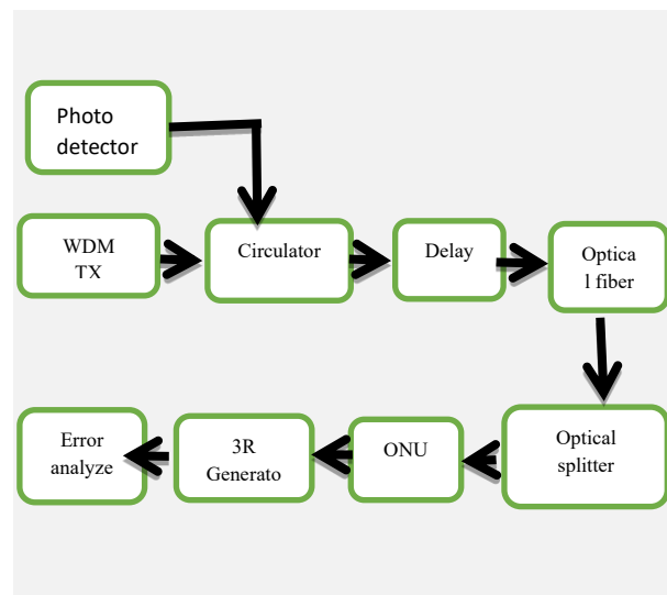
Figure 2 Block Diagram of PON
