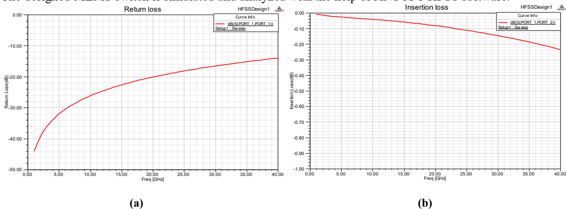
Fig.5. Simulated Result of RF MEMS Capacitive Shunt Switch in ON-state (a) Return Loss and (b) Insertion Loss
